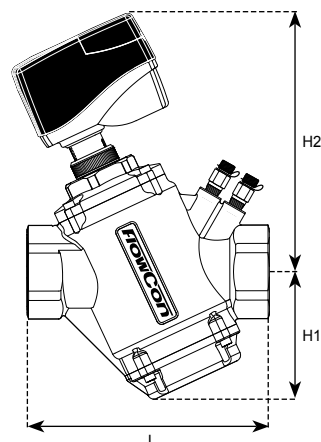
FlowCon Green DN40/50 (1 1/2"-2") with FlowCon FH actuator
